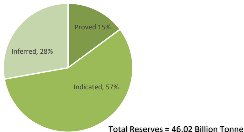
Fig 1.2 Estimated Reserves of Lignite as on 01.04.2020
