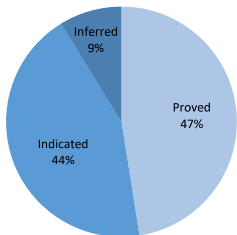
Fig 1.1 Estimated Reserves of Coal as on 01.04.2020
