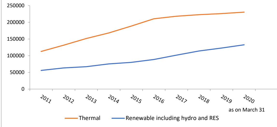
Fig 2.2: Yearwise Installed Capacity of Electricity Generation from Utilities (MW) - Source Wise
